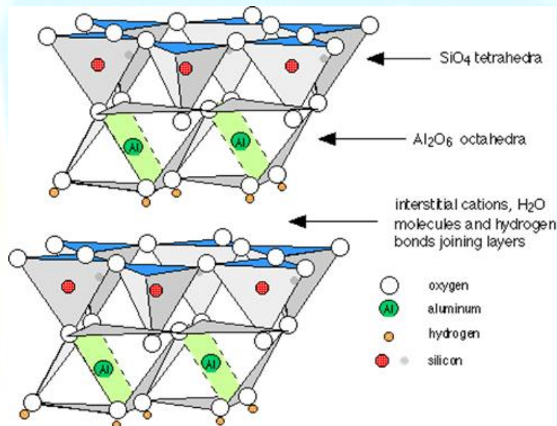
Fig.1. Molecular structure of bentonite
